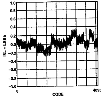
Figure 3. Typical INL
