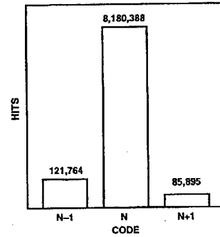
Figure 4. "Grounded-Input" Histogram (Input Span = 2 V p-p)
