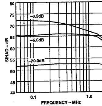
Figure 7. SINAD vs. Input Frequency (Input Span = 5.0 V p-p, V_{CM} = 2.5 V)
