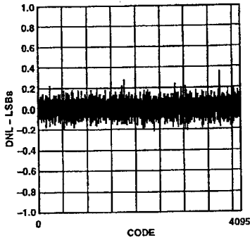
Figure 2. Typical DNL
