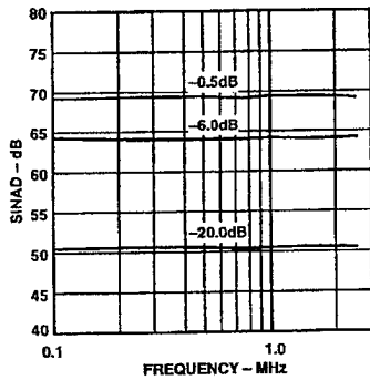
Figure 5. SINAD vs. Input Frequency (Input Span = 2.0 V p-p, V_{CM} = 2.5 V)
