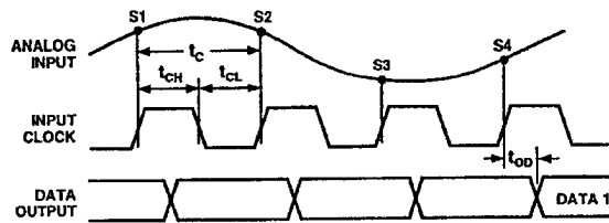
Figure 1. Timing Diagram
